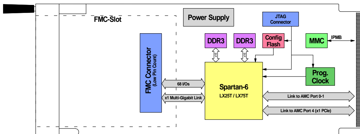
Figure 1-1 : Block Diagram
