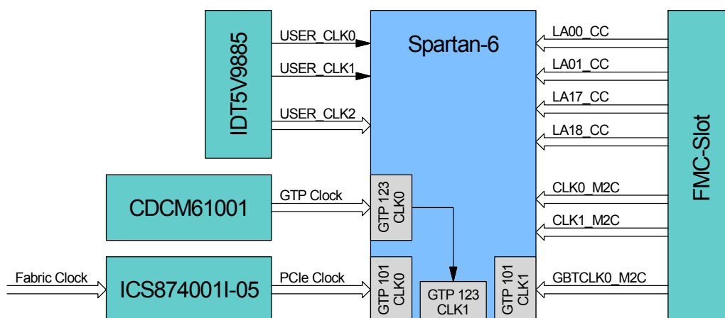
Figure 5-5 : FPGA Clock Sources
