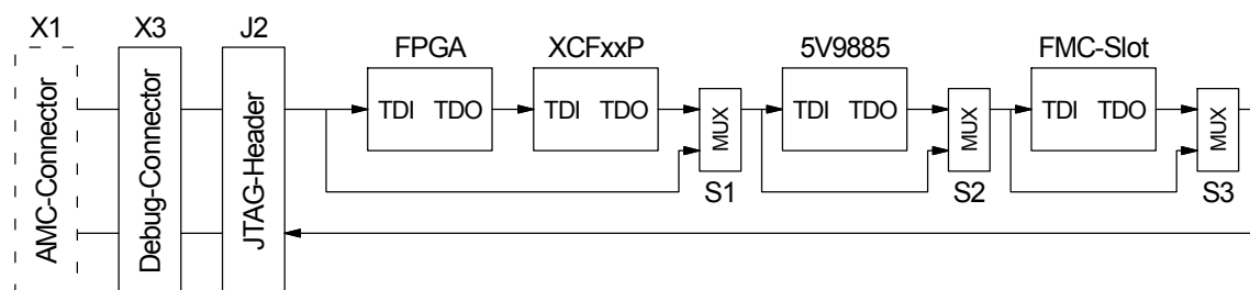
Figure 5-3 : JTAG-Chain Segmentation
