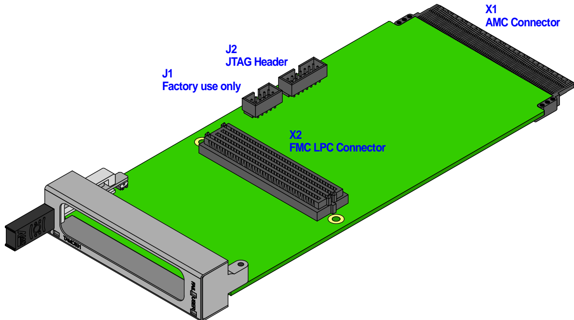
Figure 8-1 : Connector Positions
