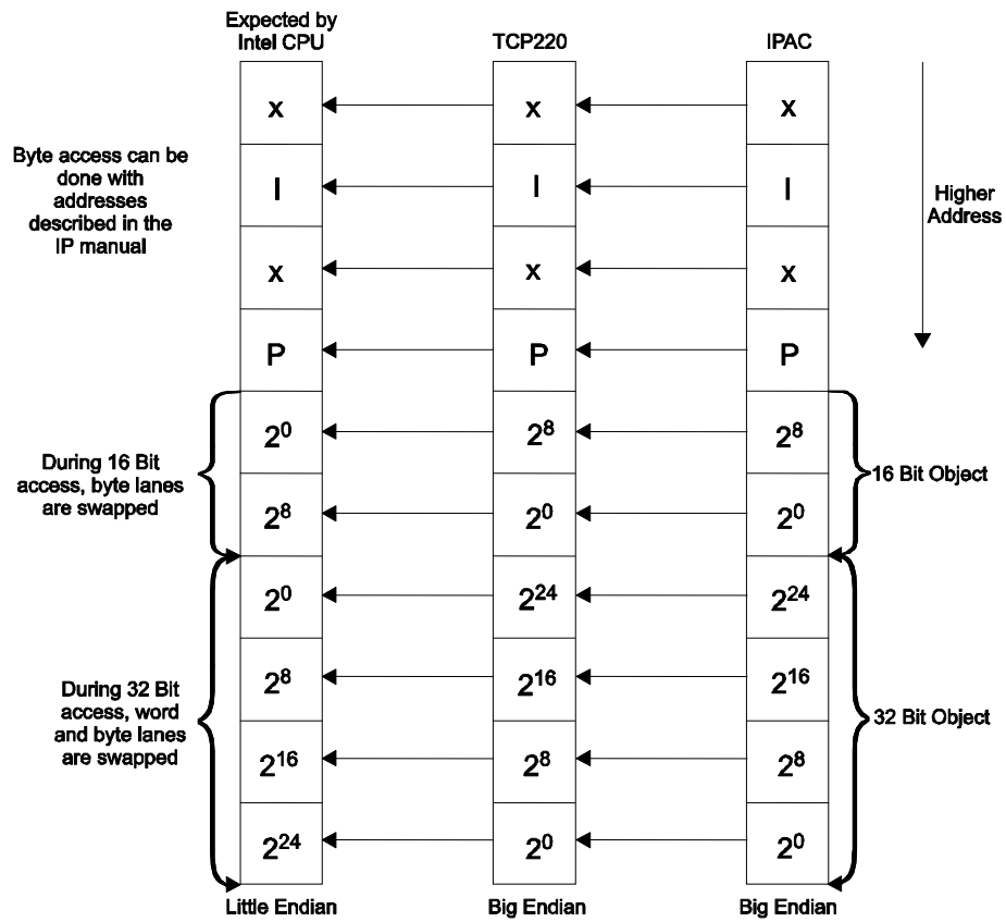
Figure 3-6 : Intel CPU View with TCP220 switched to Big Endian
