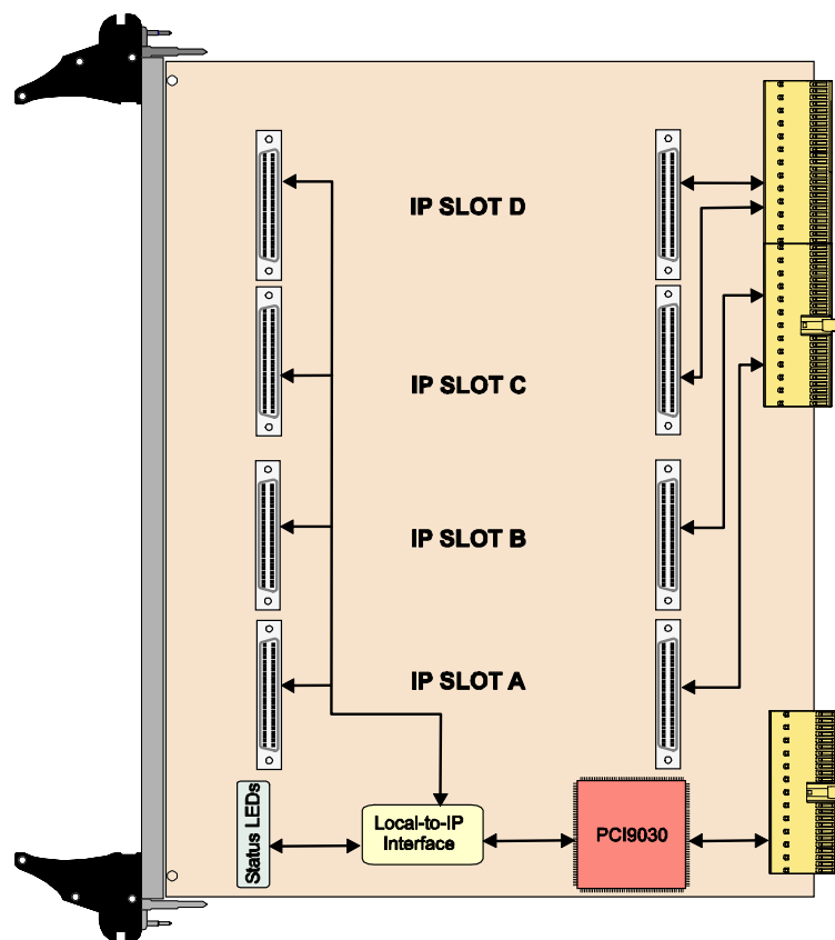
Figure 1-1 : Block Diagram
