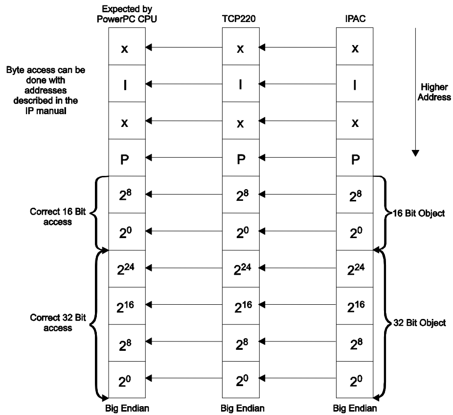
Figure 3-7 : PowerPC CPU View with TCP220 switched to Big Endian
