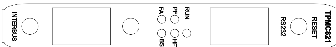
Figure 7-2 : LED Location
