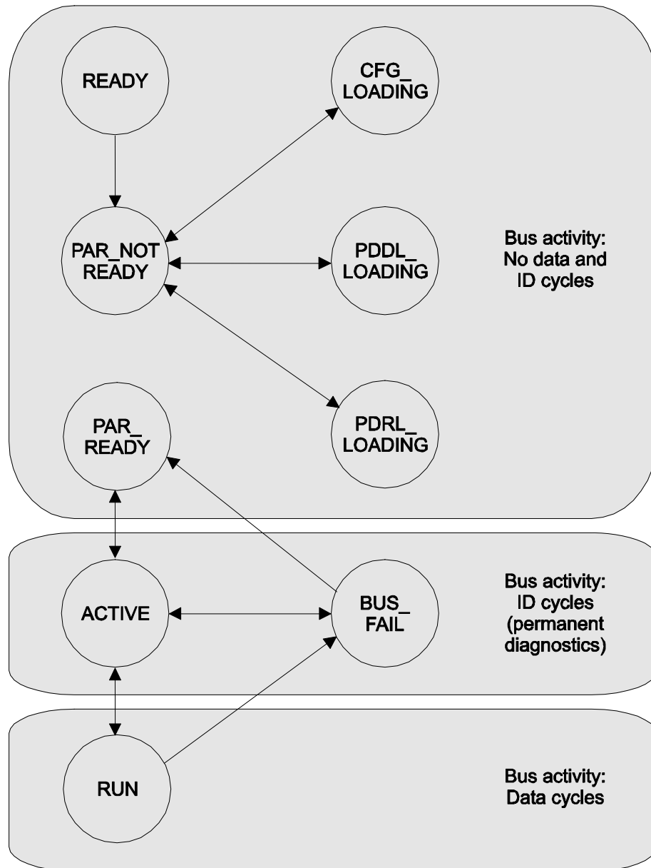
Figure 6-1 : State Machine
