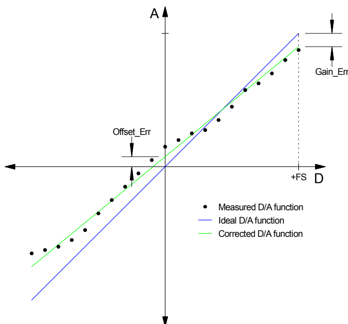
Figure 7-1 : Principle of D/A correction
